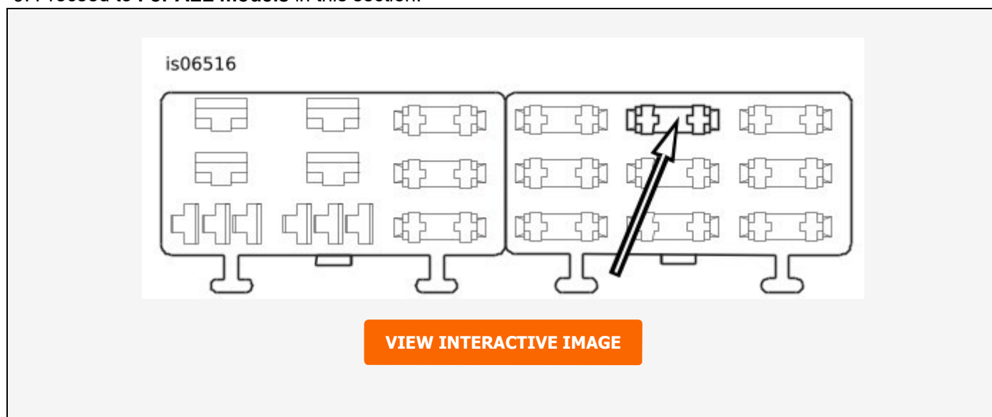
Figure 9. "P&A IGN" Fuse Block Cavity (2004-2010 Softail)
