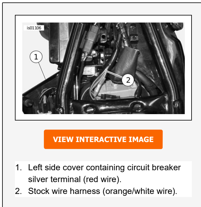
Figure 10. Power Connections (XL Models)
