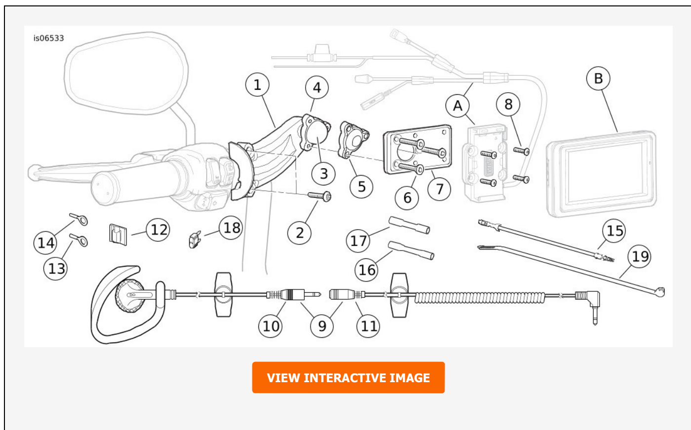
Figure 16. Service Parts, Road Tech Zumo 660 and Zumo 665 GPS Handlebar Mount Kit
