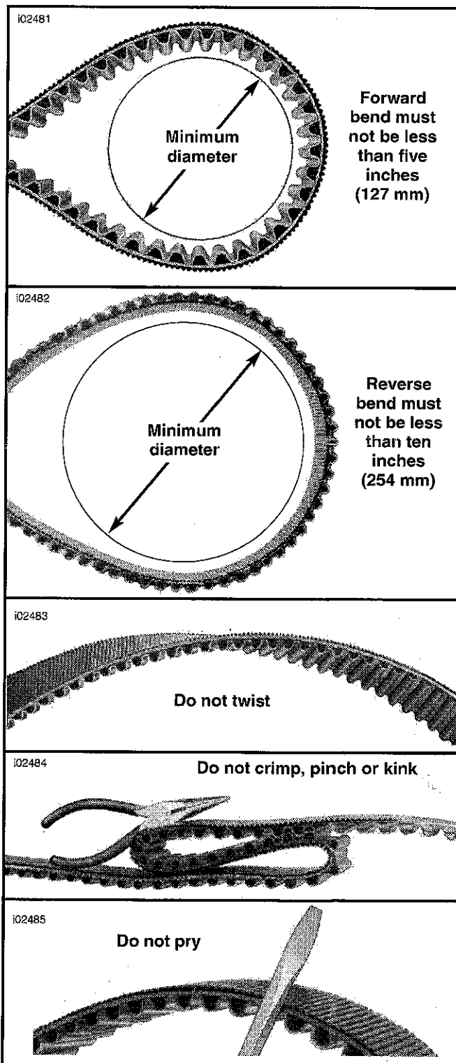
Figure 1. Proper Drive Belt Handling
